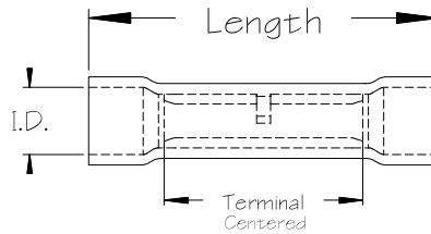
Extruded Vinyl Insulated Seamless Butt Connector
